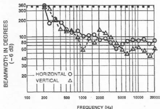
FIGURE 5 — DML-1122/DMC-1122 Beamwidth vs. Frequency Whole Space (anechoic)
