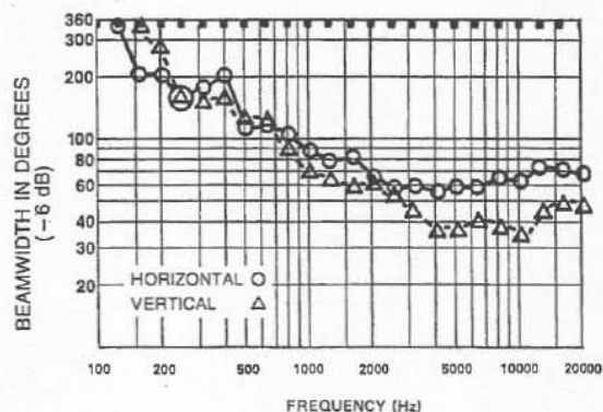
FIGURE 6 — DML-1152/DMC-1152 Beamwidth vs. Frequency Whole Space (anechoic)
